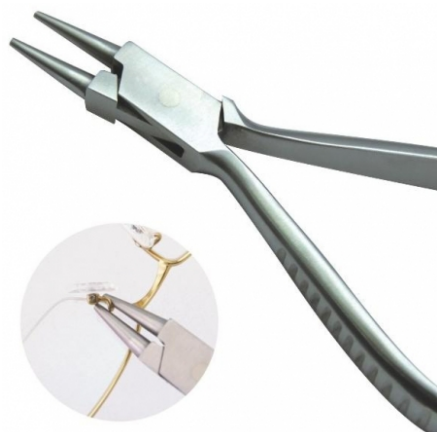
Round Snipe Nose Pliers AK-01-126 General use to adjust bridges, nose pads and joints. Intended to bend very small curves. Length: approx. 150 mm Jaws Tip: Diameter 1.2 mm Weight: approx. 117 g
